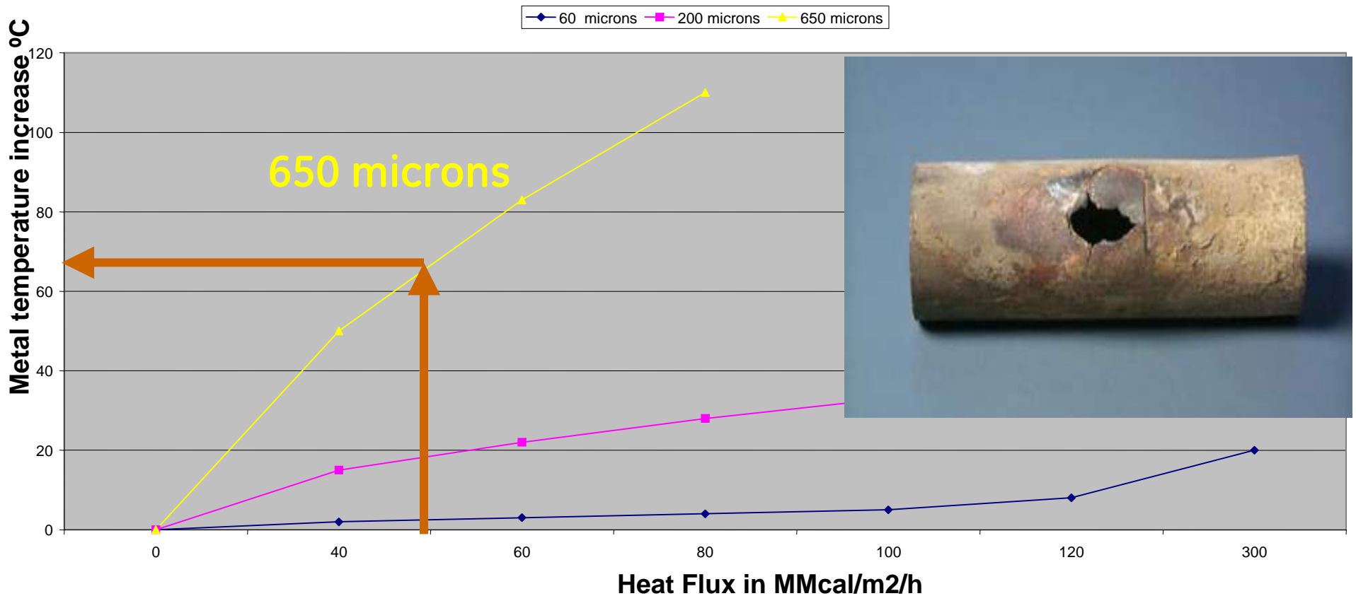
Magnetite Layer Thickness effect to metal temperature
