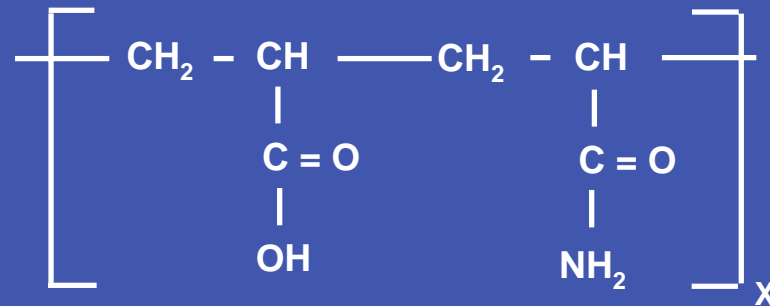
ACRYLATE-ACRYLAMIDE COPOLYMER
