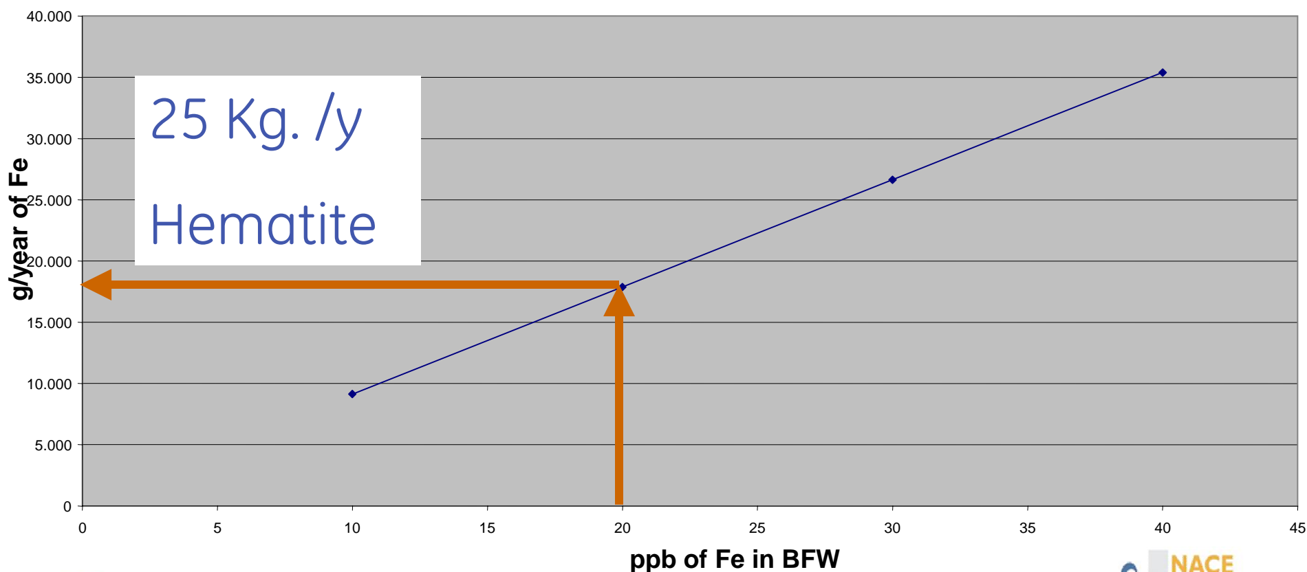
Iron introduced per year in a Boiler with BFW of 100 tn/h
