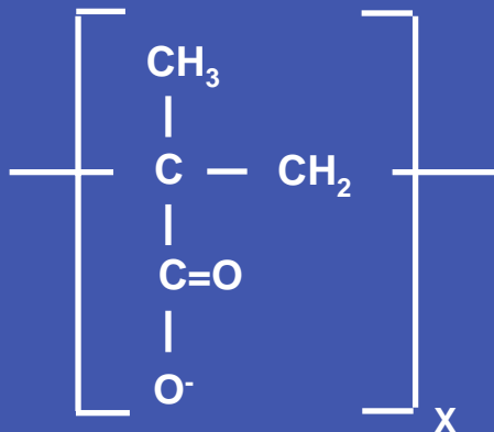
POLYMETHACRYLATE
