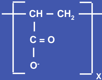
POLYACRYLATE
